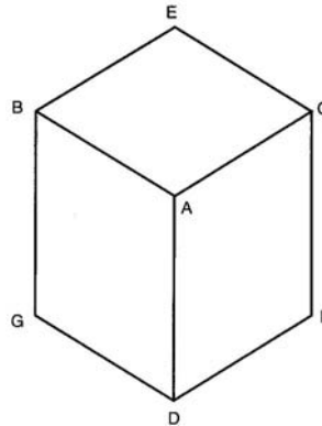
Figure 17.1: A Cube
